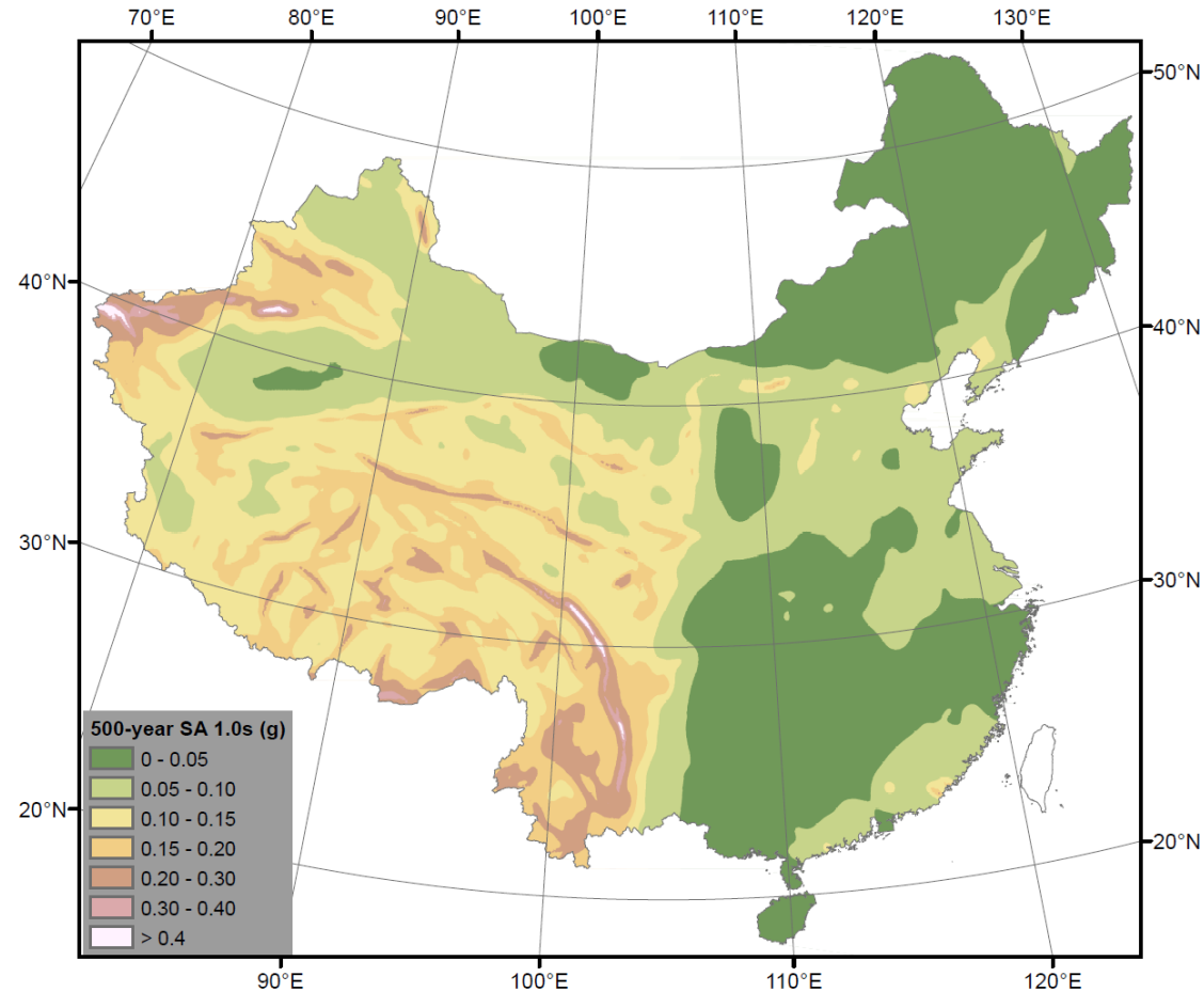
Before site amplification is considered
