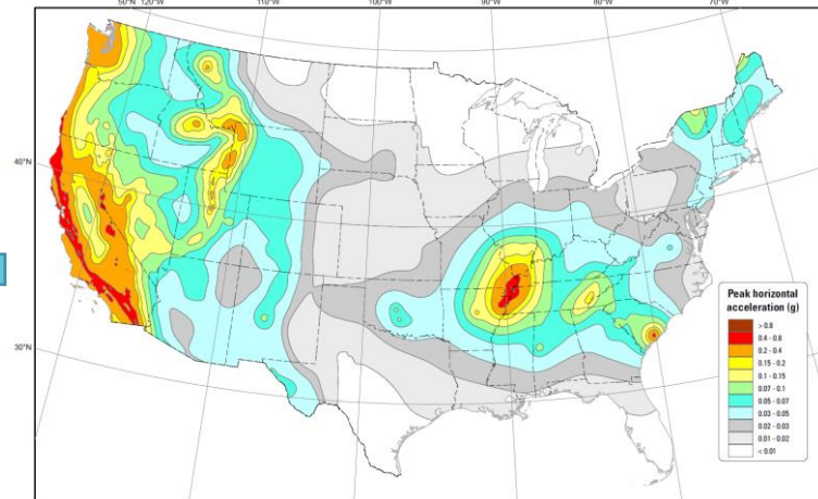
2018 national model for Conterminous United States
