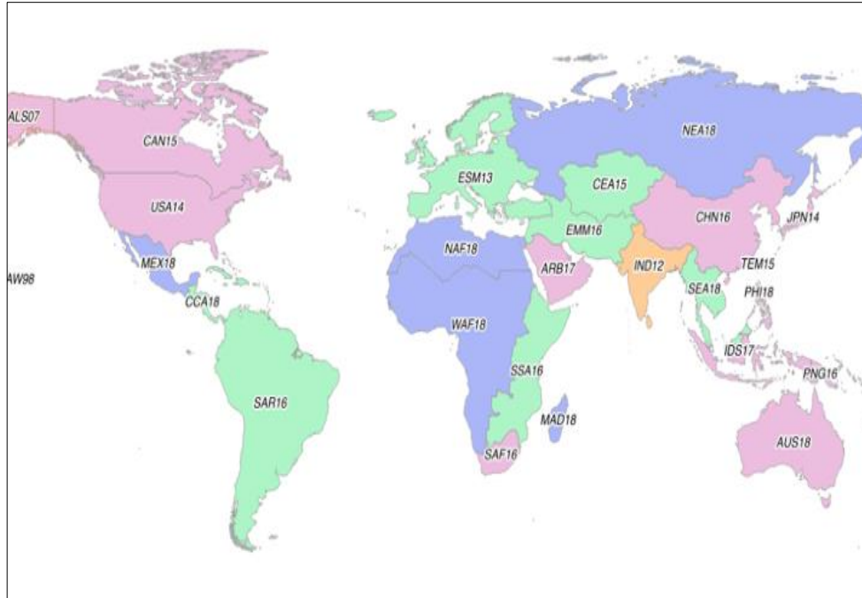
GEM mosaic hazard models
