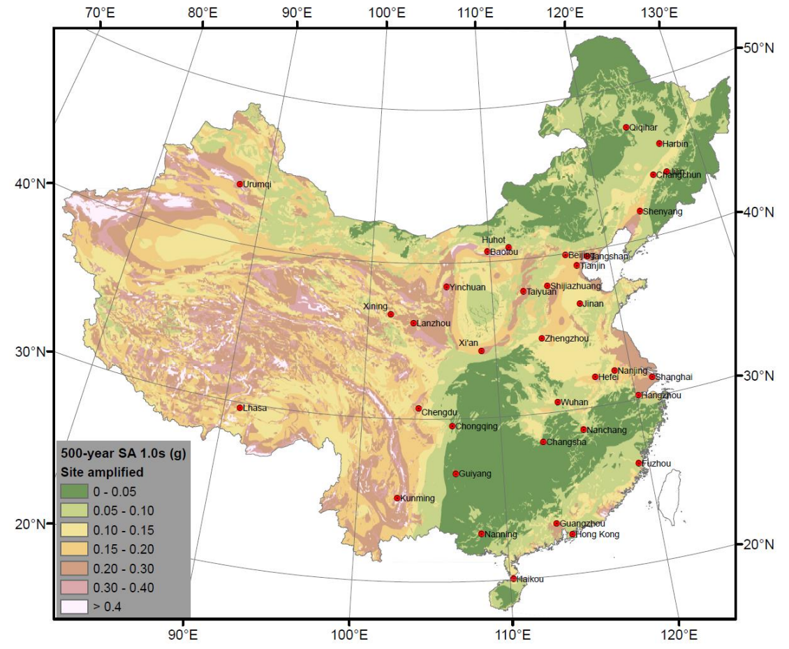
After site amplification is considered
