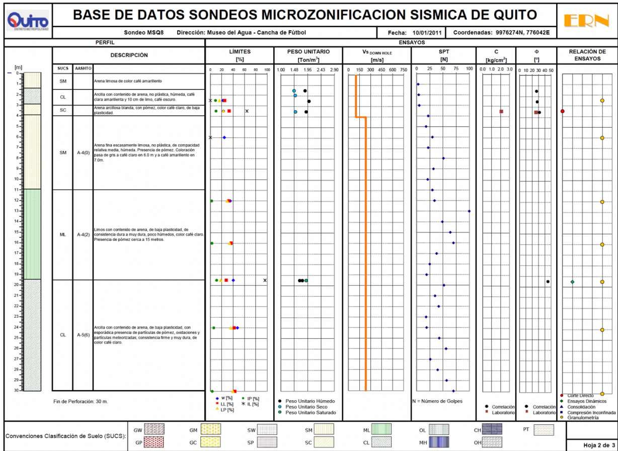
Figure 2: Example of a bore log in Quito at site MSQ8 from ERN (2012).
